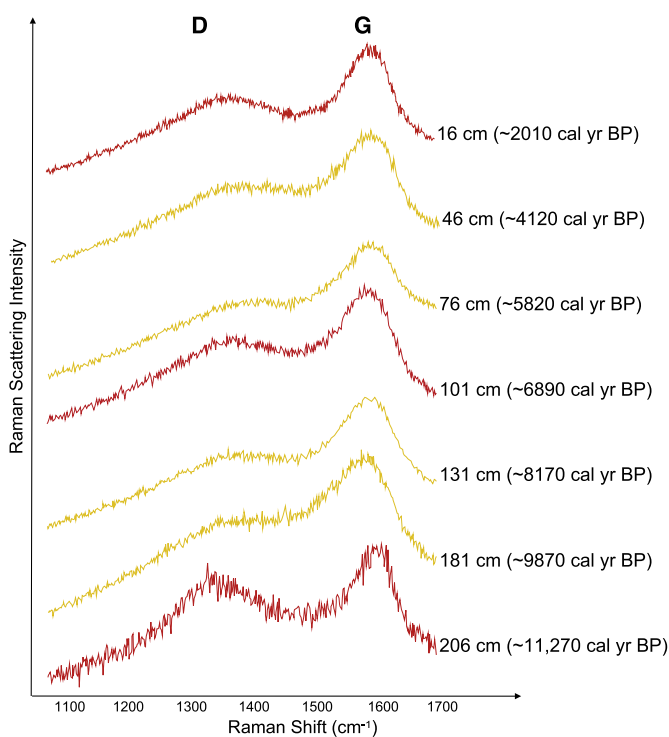
Fig. 4. Raman scattering intensity vs. Raman shifts. D = disorder peak, G = graphite peak. The three highest intensity fires from the seven samples (at 206, 101 and 16 cm depth) are filled with red, the remainder indicate lower intensity fires (filled with orange). (For interpretation of the references to colour in this figure legend, the reader is referred to the Web version of this article.)
