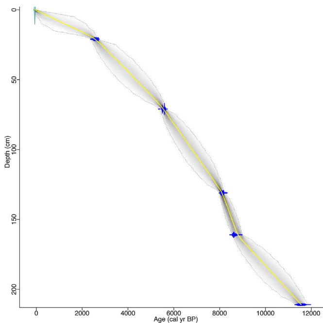
Fig. 2. Bacon age depth model. The accumulation rate prior was set to 50 years \text{cm}^{-1} with a shape of 1.5. The memory prior was set to a strength of 4 and a mean of 0.7. The model is based upon 43 sections (5 cm thick).
