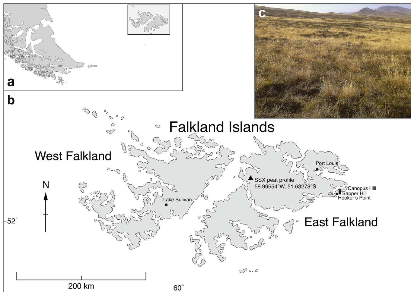
Fig. 1. a. location of the Falkland Islands/Islas Malvinas in the South Atlantic Ocean, b. site locations: Sussex Mountains (SSX, 58.99654°W, 51.63278°S) peat profile (black triangle), other sites mentioned in the text (black squares), Canopus Hill (Turney et al., 2016), Hooker's Point (Scaife et al., 2019), Lake Sullivan (Wilson et al., 2002), Sapper Hill (Buckland and Edwards (1998) c. photograph of the SSX peat profile coring location.
