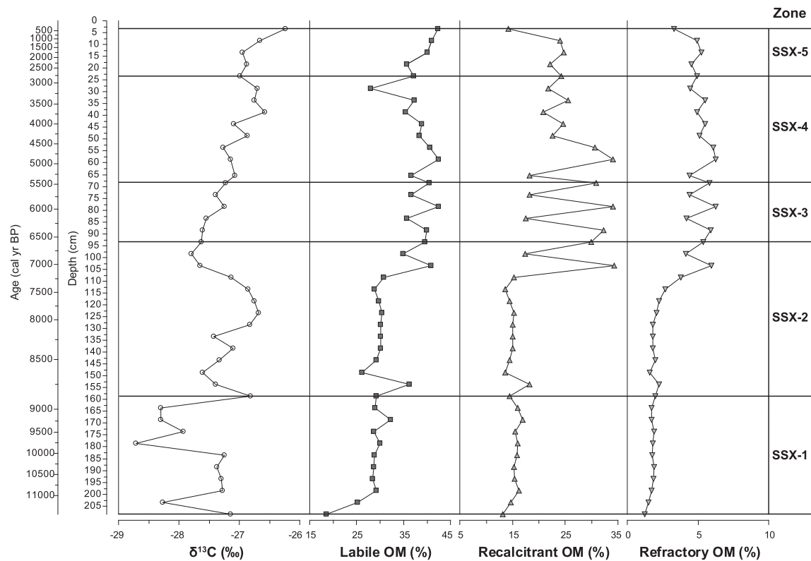
Fig. 5. \delta^{13}\text{C} and TGA, OM mass loss data grouped into three thermal fractions: labile (200–400 °C), recalcitrant (400–550 °C) and refractory (550–650 °C). The zonation is based upon the loss-on-ignition, plant macrofossil and macrofossil charcoal data.
